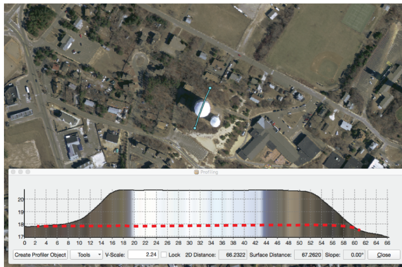
Figure 6. Example of ‘pull up’ near a water tower. Dotted line is more representative of elevations at the water tower. Blue line in image is location in profile. Profile units = meters (Vert. NAVD88, Hor. NAD83).
