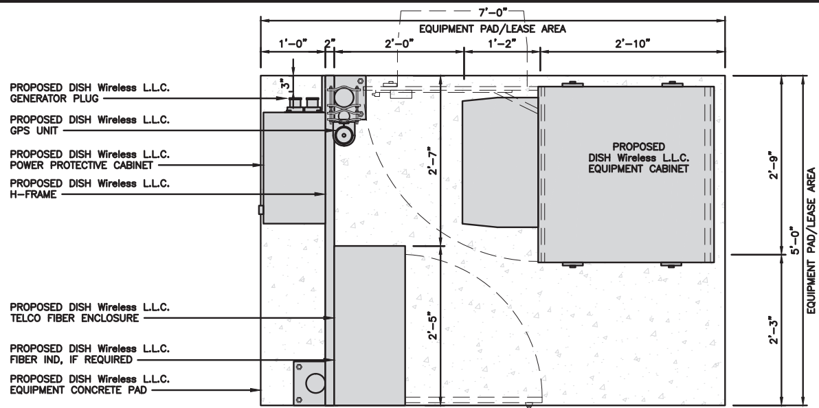
EQUIPMENT PLAN
