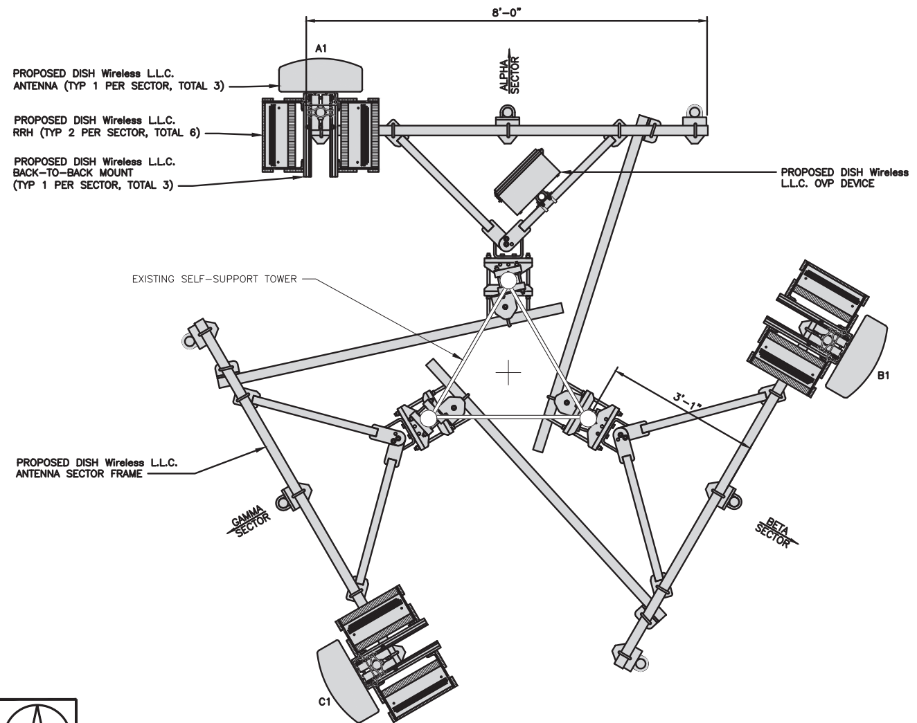
ANTENNA LAYOUT
