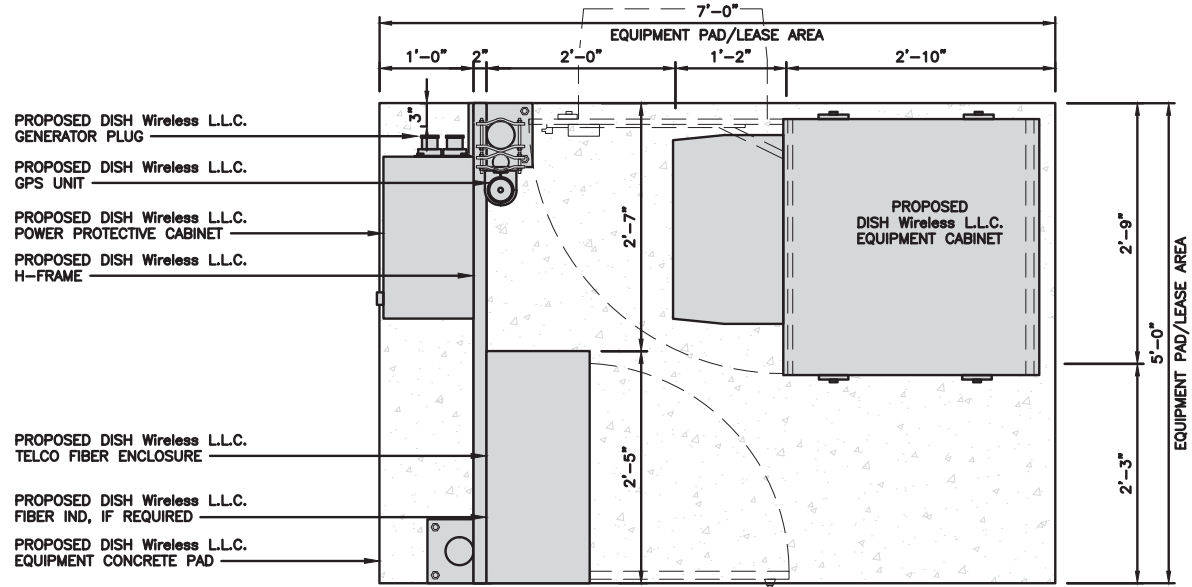
EQUIPMENT PLAN
